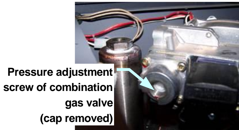
Illustration 3 - Gas Valve Adjustment Screw
